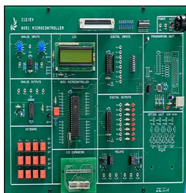
MicroController
