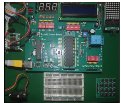
AVR Trainer Board
